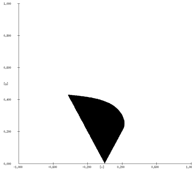
Figure 4.1: Numerically determined invariance kernel \text{Inv}_\psi(D) for System (4.1), W = \mathbb{R}
