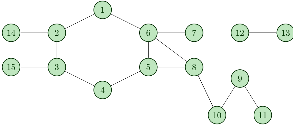
Figure 7.5: Example of a graph
