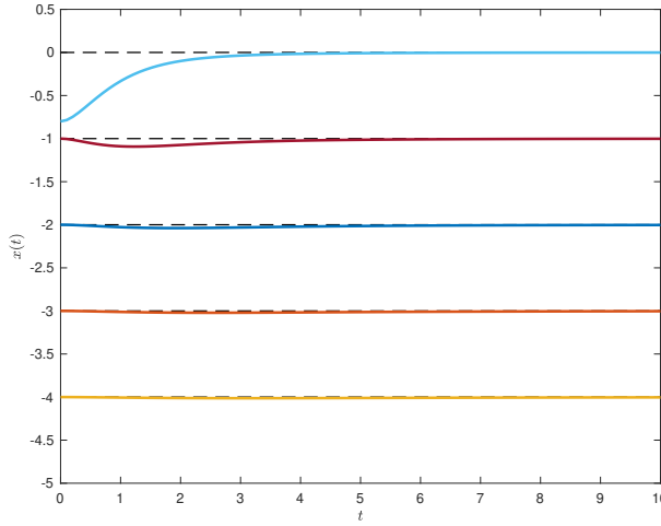
Figure 7.4: Deviation of vehicle positions from their desired places
