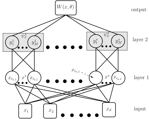
Figure 7.1: Neural network with separable structure
